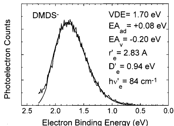
Figure 5. Best fit of the dimethyl disulfide photoelectron spectrum obtained, using energetic and structural parameters as indicated and an estimated anion temperature of 150 K.
